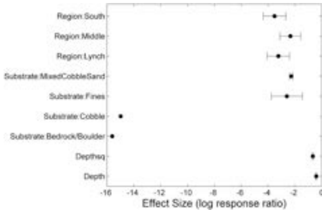
Figure 4. Estimated coefficients (SE) from the generalized linear model depicting the effect of depth, depth squared (Depthsq), region, and substrate on geoduck densities. Coefficients are log-response ratios, and within categorical variables are expressed as a log-ratio relative to a reference level within that category. Reference levels were sand and North for substrate and region, respectively.
